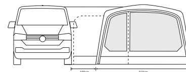
Shown with optional Movelite polycotton Zip on Porch Door & annexe
