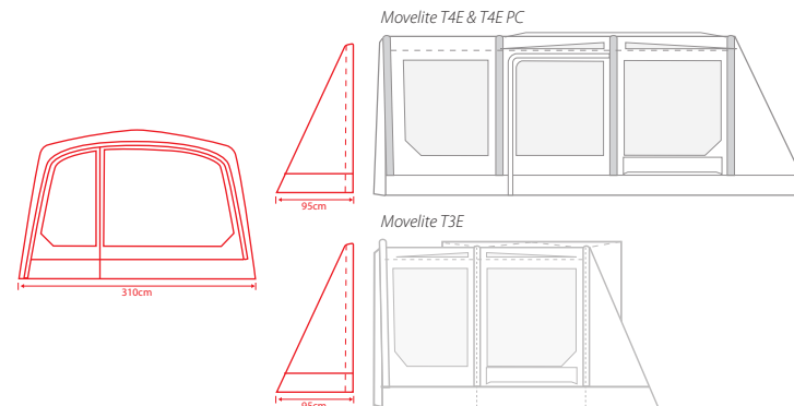
Movelite Polycotton Zip on Porch Door shown on Movelite T4E PC
